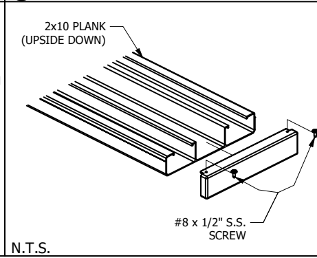
② TYPICAL 2 X 10 END CAP ATTACHMENT
