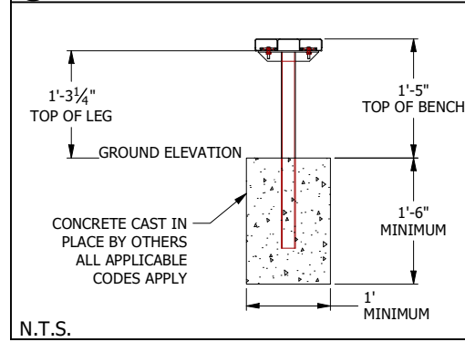
① BE-DD BENCH CONCRETE EMBEDMENT
