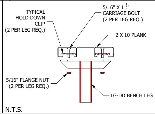
③ TYPICAL 2 X 10 PLANK ATTACHMENT
